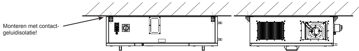
Afb.4: Apparaatophanging
